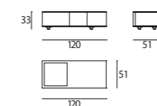
ESOV120B Storage table cm.120x51x33
