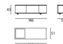
ESOV146A Storage table cm.146x51x43
